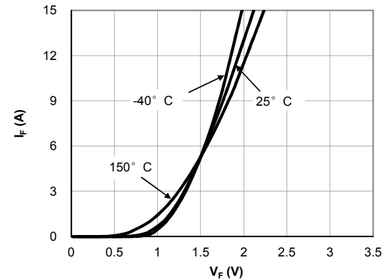
Figure 4: Diode Characteristic
